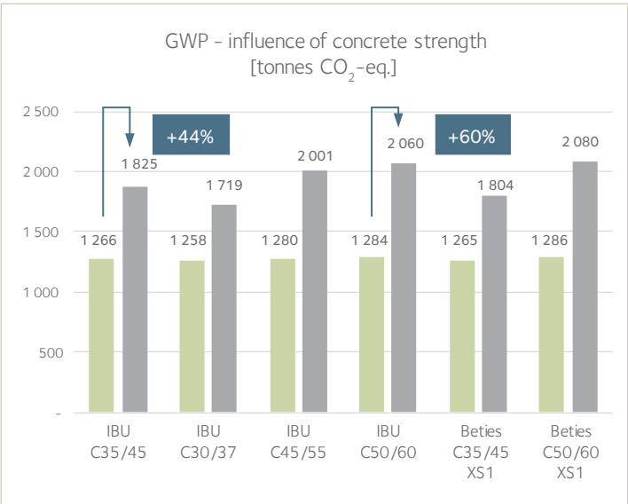
Figure 6. Global Warming Potential - Total value (tonnes of CO 2 -eq.) Scenario with different concrete strengths
